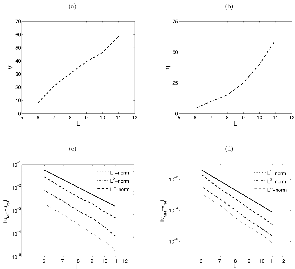
Fig. 12. Example 4 (model 2 with non-degenerate diffusion): (a) CPU acceleration V , (b) data compression rate \eta , for different levels, at time t = 0.75 s, (c) errors \|\tilde{u}_{MR} - \tilde{u}_{ref}\|_1 , \|\tilde{u}_{MR} - \tilde{u}_{ref}\|_2 , \|\tilde{u}_{MR} - \tilde{u}_{ref}\|_\infty and (d) \|\tilde{v}_{MR} - \tilde{v}_{ref}\|_1 , \|\tilde{v}_{MR} - \tilde{v}_{ref}\|_2 and \|\tilde{v}_{MR} - \tilde{v}_{ref}\|_\infty respectively for different levels L , at time t = 0.75 . The thick solid line in plots (c) and (d) is the theoretical slope of a convergence rate 2.
