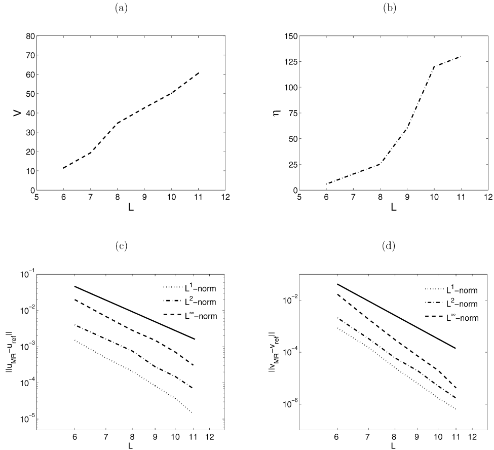
Fig. 8. Example 2 (interaction of two flame balls without radiation): (a) speed-up rate V , (b) data compression rate \eta , for different levels, at time t = 4.0 ; (c) errors \|\tilde{u}_{MR} - \tilde{u}_{ref}\|_1 , \|\tilde{u}_{MR} - \tilde{u}_{ref}\|_2 , \|\tilde{u}_{MR} - \tilde{u}_{ref}\|_\infty and (d) \|\tilde{v}_{MR} - \tilde{v}_{ref}\|_1 , \|\tilde{v}_{MR} - \tilde{v}_{ref}\|_2 and \|\tilde{v}_{MR} - \tilde{v}_{ref}\|_\infty respectively for different levels L , at time t = 4 . The thick solid line in plots (c) and (d) is the theoretical slope of a convergence rate 2.
