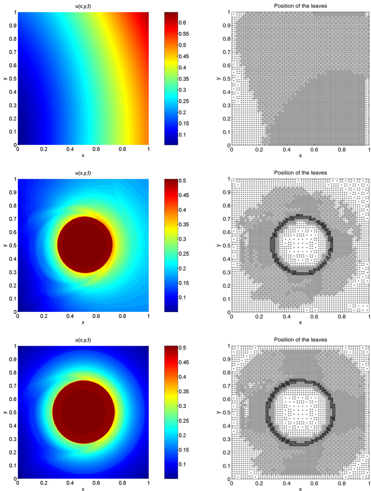
Fig. 3. Example 1 (single-species model): numerical solution (left) and leaves of the tree data structure (right) at times t=0 (top), t=0.5 (middle) and t=3 (bottom).
