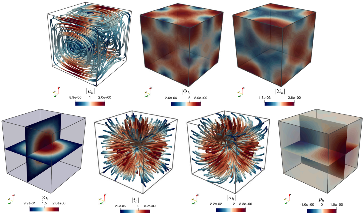
Fig. 2. Example 1. Approximate solutions for the 3D manufactured problem with \ell = 2 : velocity streamlines, strain rate magnitude, pseudostress magnitude, slices of concentration profile, diffusive flux and total flux streamlines, and slices of postprocessed pressure.
