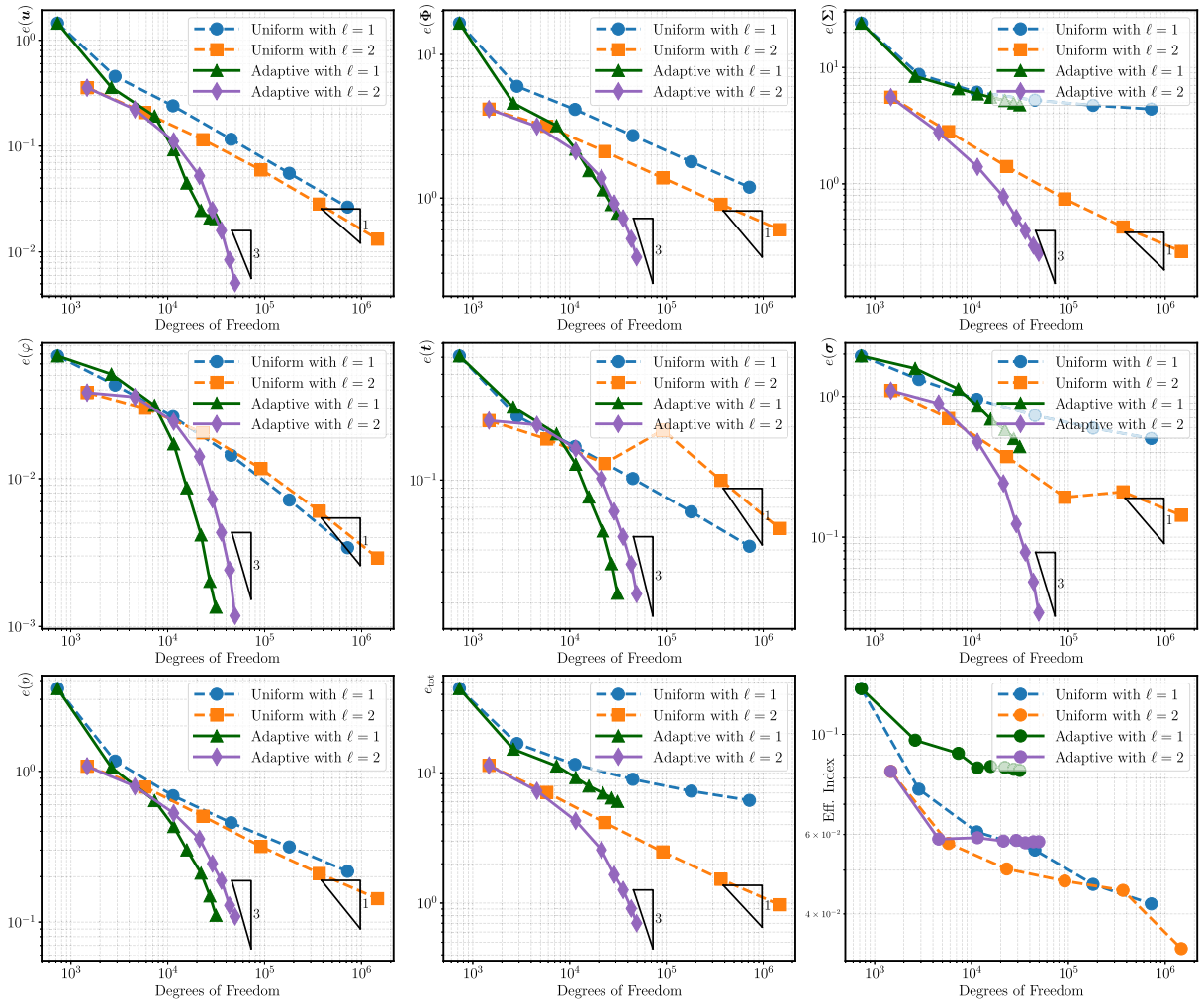
Fig. 3. Example 2. Convergence for each field variable against non-smooth solutions on an L-shaped domain using uniform and adaptive mesh refinement with barycentrically refined meshes. The bottom right plot shows effectivity indexes for all cases. For reference we show triangles indicating linear and cubic slopes.
