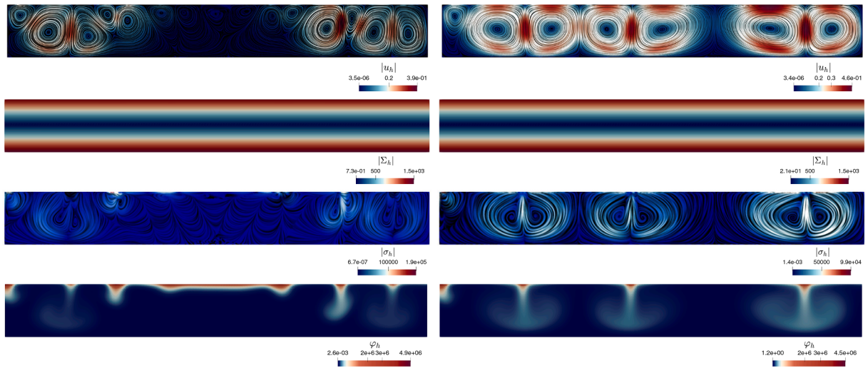
Fig. 6. Example 4. Snapshots of the numerical solution (showing here only velocity, stress magnitude, flux, and concentration) at t = 75 s (left) and t = 150 s (right).
