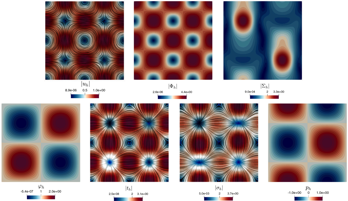
Fig. 1. Example 1. Approximate solutions for the 2D manufactured problem with \ell = 2 : velocity line integral contours, strain rate magnitude, pseudostress magnitude, concentration profile, diffusive flux and total flux magnitudes, and postprocessed pressure.
