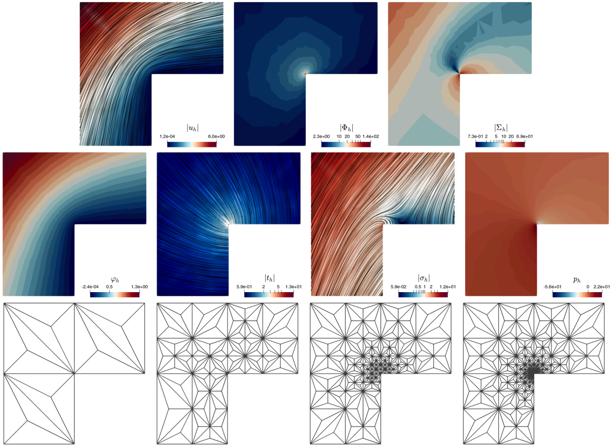
Fig. 4. Example 2. Approximate solutions for the 2D manufactured problem on an L-shaped domain with \ell = 2 and rendered on a coarse mesh: velocity line integral contours, strain rate magnitude, pseudostress magnitude, slices of concentration profile, diffusive flux and total flux line integral contours, and postprocessed pressure. The bottom row shows four adaptively refined meshes.
