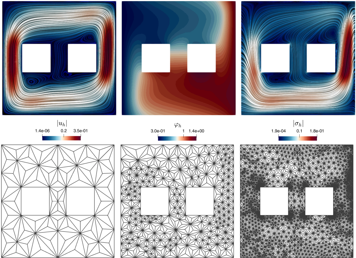
Fig. 5. Example 3. Bioconvection of micro-organisms on a cavity with square inclusions and mixed boundary conditions. Velocity line integral contours, concentration profile, and total flux line integral contours for the case \alpha = 0.3 . The bottom row shows three samples of adaptively refined meshes.
