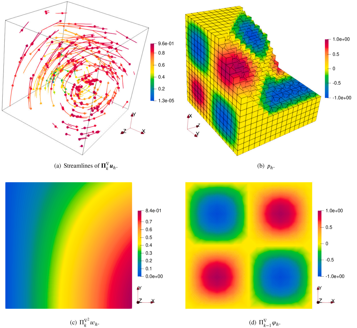
Fig. 4. Example 1. Snapshots of the variables of interest for the Octa mesh in the last refinement step.
