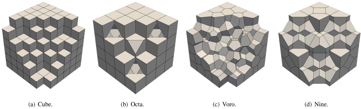
Fig. 3. Example 1. Cross-section of a variety of meshes used in the accuracy verification test.
