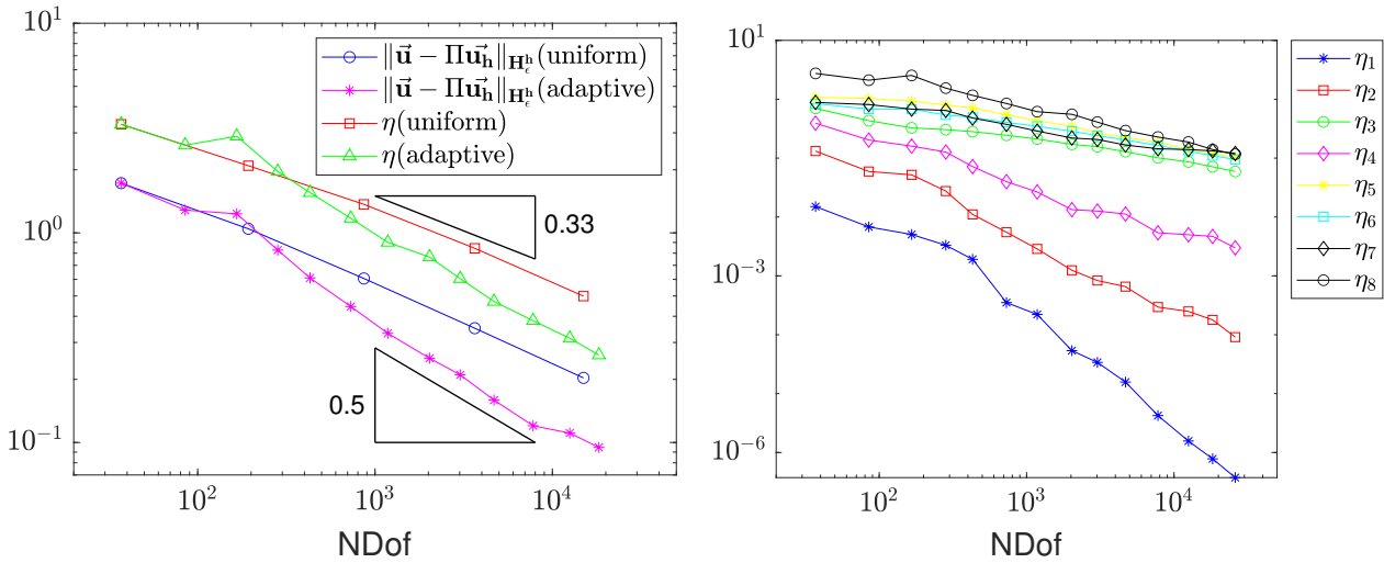
Figure 7.7: Left panel displays NDof vs error in energy norm and estimator in both uniform and adaptive refinements, and right panel displays estimator components in adaptive refinement for non-conforming VEM.
