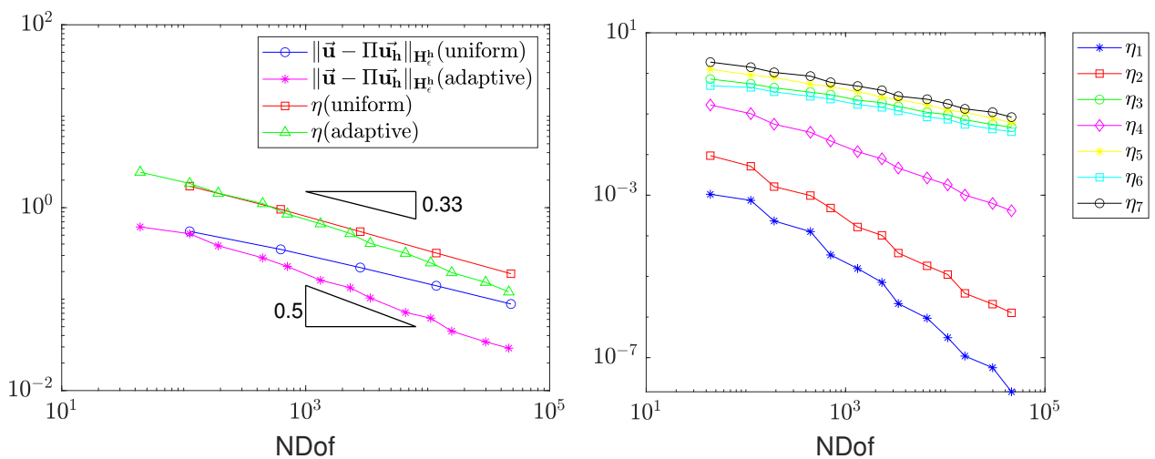
Figure 7.6: Left panel displays NDof vs error in energy norm and estimator in both uniform and adaptive refinements, and right panel displays estimator components in adaptive refinement for conforming VEM.
