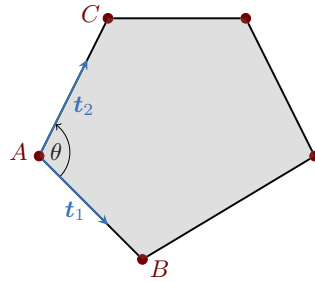
Figure 6.1: Sketch of a polygonal domain K and three consecutive vertices A, B, C . The unit vectors \mathbf{t}_1, \mathbf{t}_2 form an angle \theta on A .
