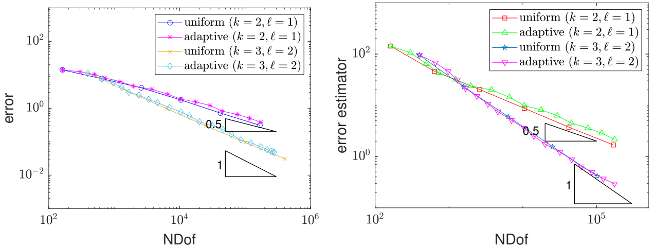
Figure 7.3: Left (resp. right) panel displays NDof vs error in energy norm (resp. error estimator) in both uniform and adaptive refinements for nonconforming VEM.
