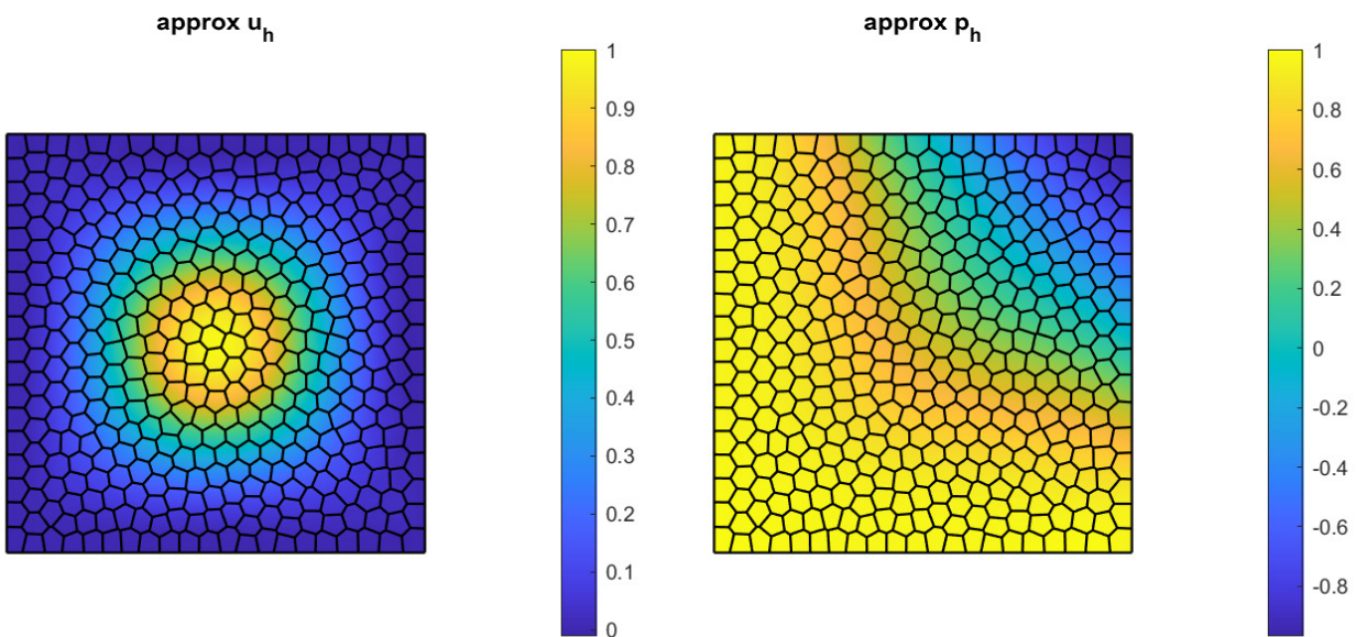
Figure 7.1: Approximation u_h of displacement u for k = 2 (left) and p_h of pressure p for \ell = 1 (right) on a smooth Voronoi mesh of 400 elements.
