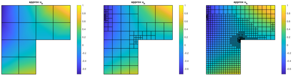
Figure 7.4: Approximation u_h of displacement u on adaptive meshes \mathcal{T}_1, \mathcal{T}_5, \mathcal{T}_{10} .
