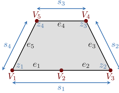
Figure 3.1: Sample of pentagonal element with vertices V_1, \dots, V_5 , edges e_1, \dots, e_5 , corners z_1, \dots, z_4 , and sides s_1, \dots, s_4 .
