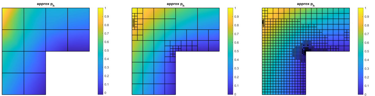
Figure 7.5: Approximation p_h of pressure p on adaptive meshes \mathcal{T}_1, \mathcal{T}_5, \mathcal{T}_{10} .
