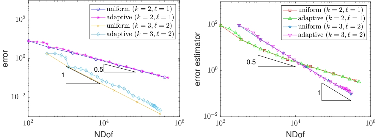
Figure 7.2: Left (resp. right) panel displays NDof vs error in energy norm (resp. error estimator) in both uniform and adaptive refinements for conforming VEM.
