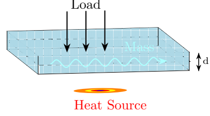
Fig 1.1: 3D plate in reference configuration.
