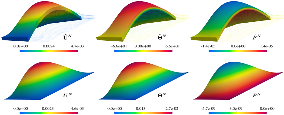
Fig 5.2: Example 1. 3D (upper) and 2D (lower) displacement , temperature, and chemical potential at final time T for TED model.
